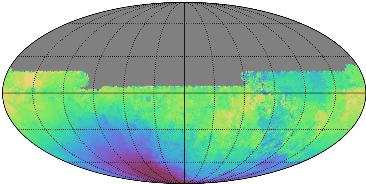
weather_cloudso0v3.5_10yrs All sky u band: Median solarElong
