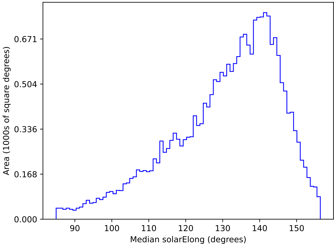
weather_cloudso0v3.5_10yrs All sky u band: Median solarElong
