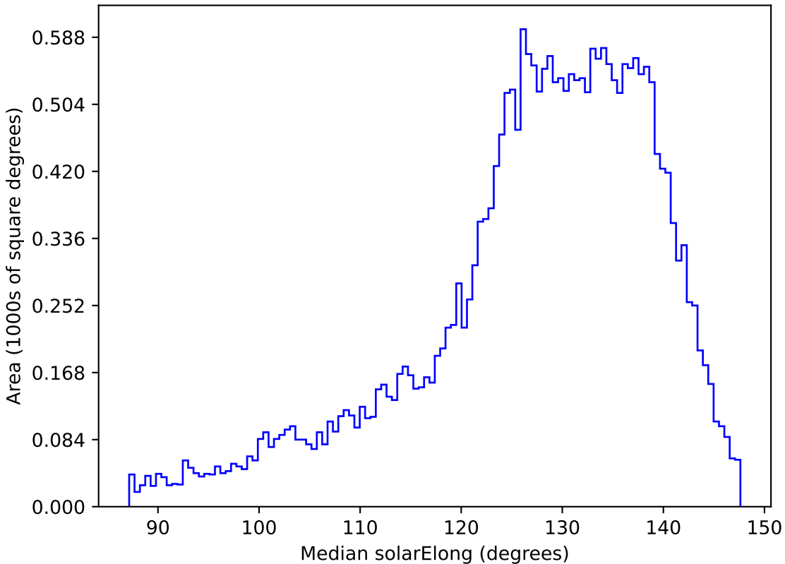
weather_cloudso0v3.5_10yrs All sky i band: Median solarElong
