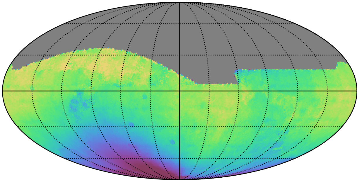
weather_cloudso0v3.5_10yrs All sky all bands: Median solarElong
