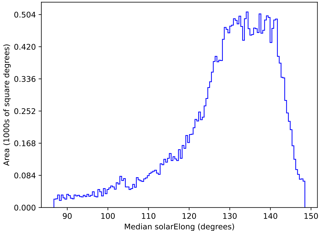
weather_cloudso0v3.5_10yrs All sky all bands: Median solarElong
