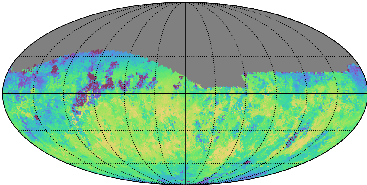
weather_cloudso0v3.5_10yrs Yr 1 z band: Median skyBrightness
