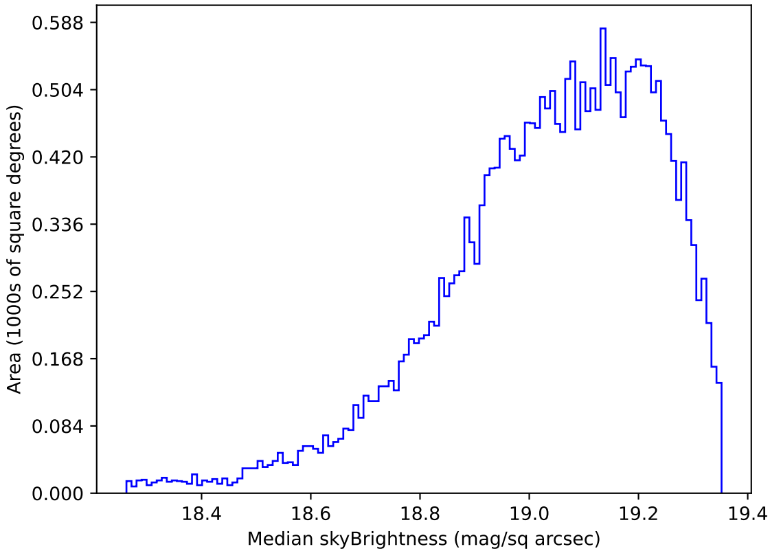
weather_cloudso0v3.5_10yrs Yr 1 z band: Median skyBrightness
