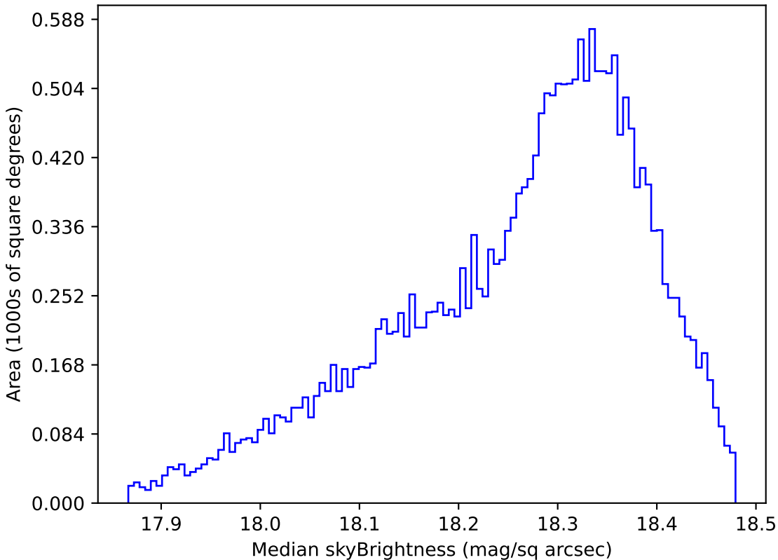
weather_cloudso0v3.5_10yrs Yr 1 y band: Median skyBrightness
