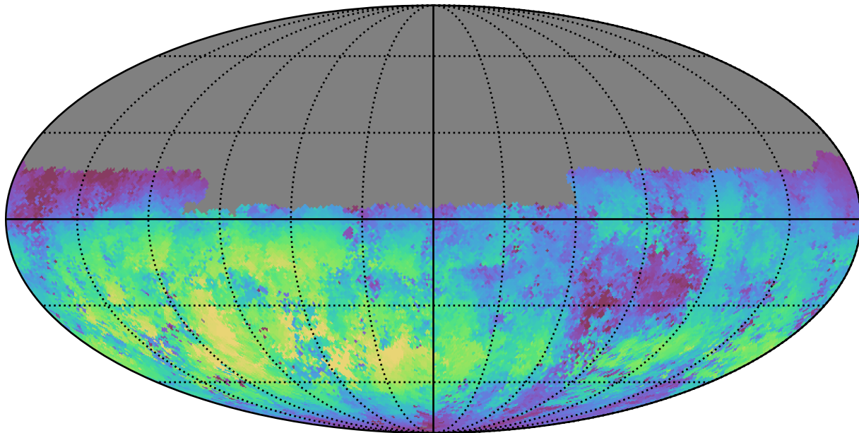
weather_cloudso0v3.5_10yrs Yr 1 u band: Median skyBrightness
