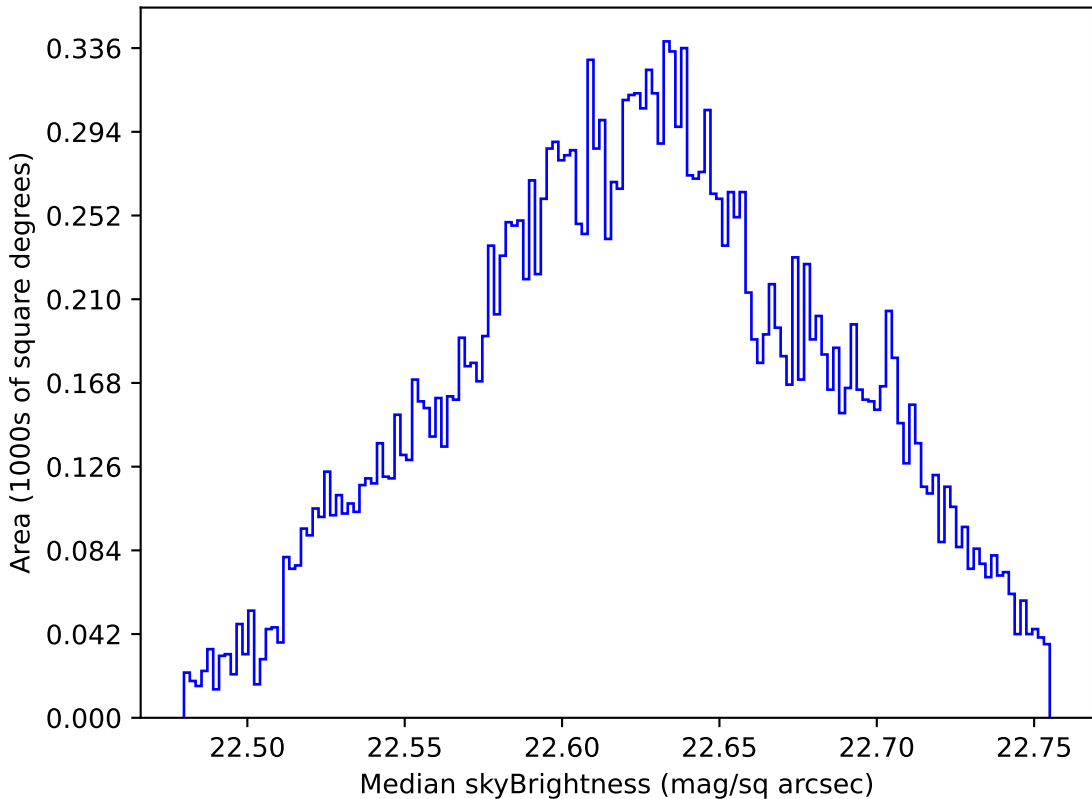
weather_cloudso0v3.5_10yrs Yr 1 u band: Median skyBrightness
