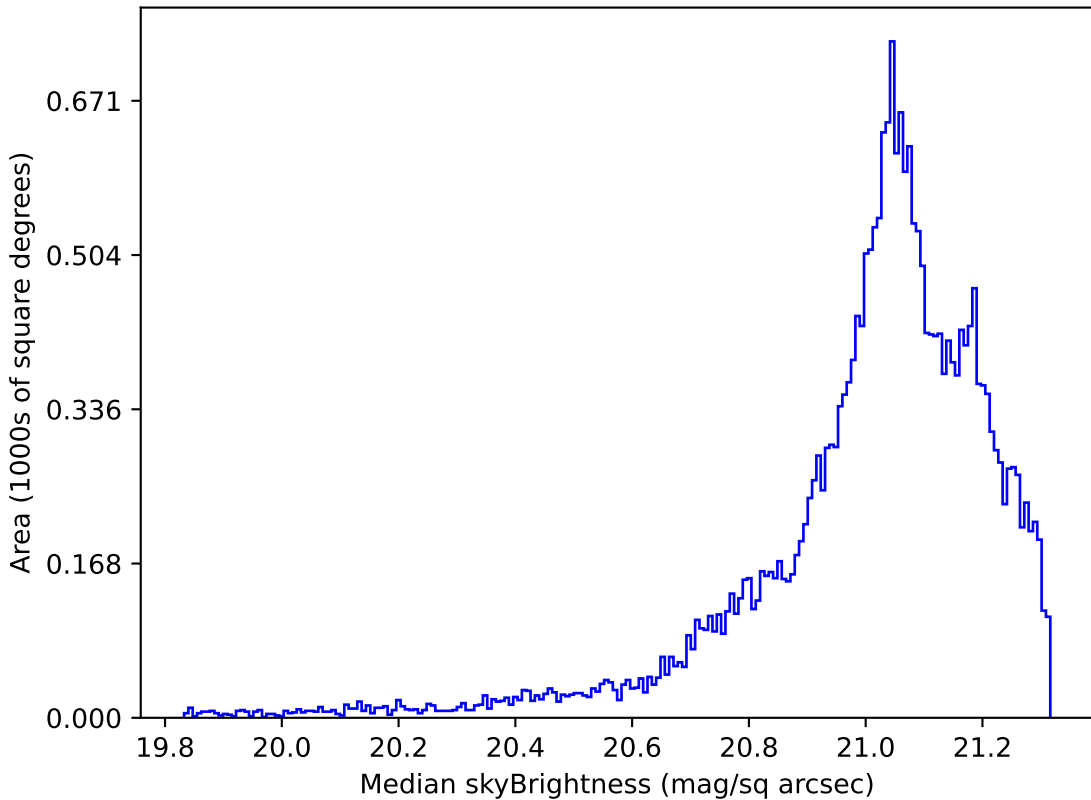
weather_cloudso0v3.5_10yrs Yr 1 r band: Median skyBrightness
