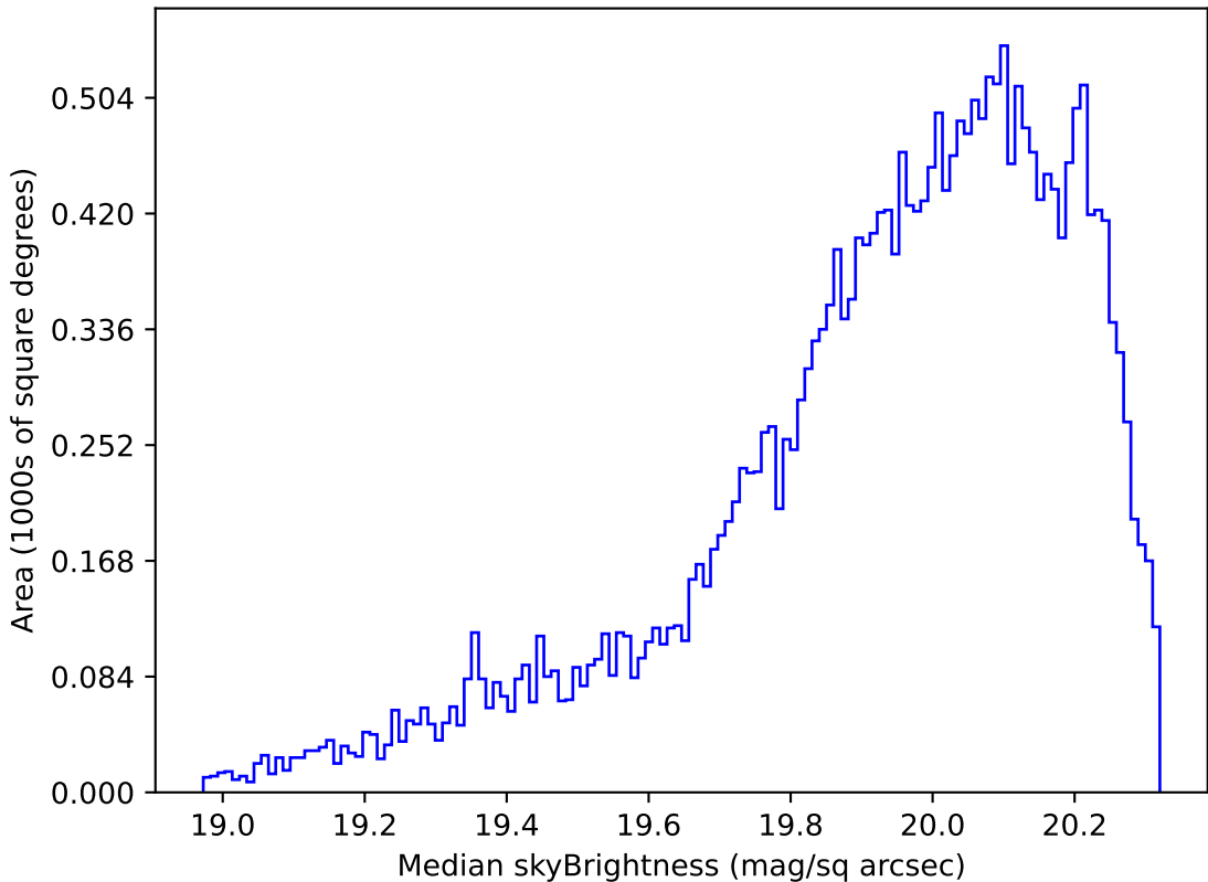
weather_cloudso0v3.5_10yrs Yr 1 i band: Median skyBrightness
