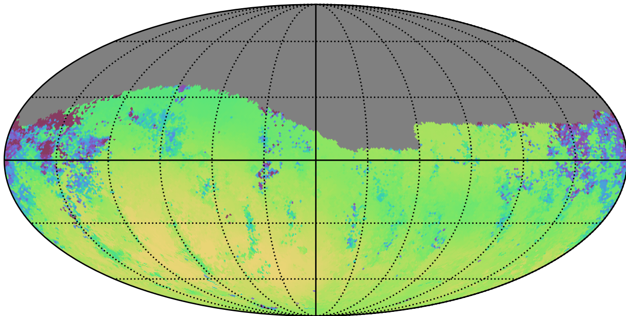
weather_cloudso0v3.5_10yrs Yr 1 g band: Median skyBrightness
