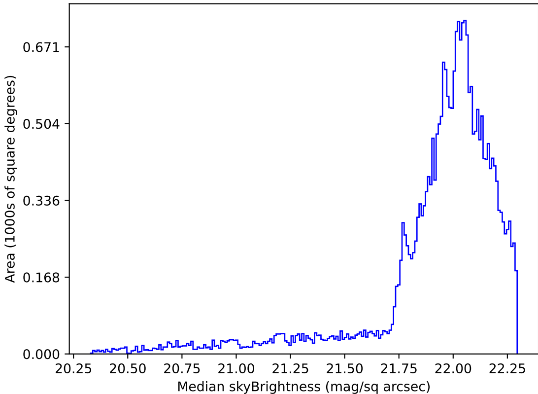
weather_cloudso0v3.5_10yrs Yr 1 g band: Median skyBrightness
