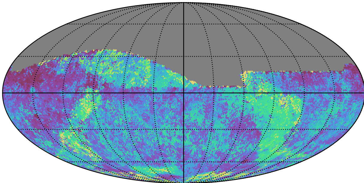
weather_cloudso0v3.5_10yrs Yr 1 all bands: Median skyBrightness
