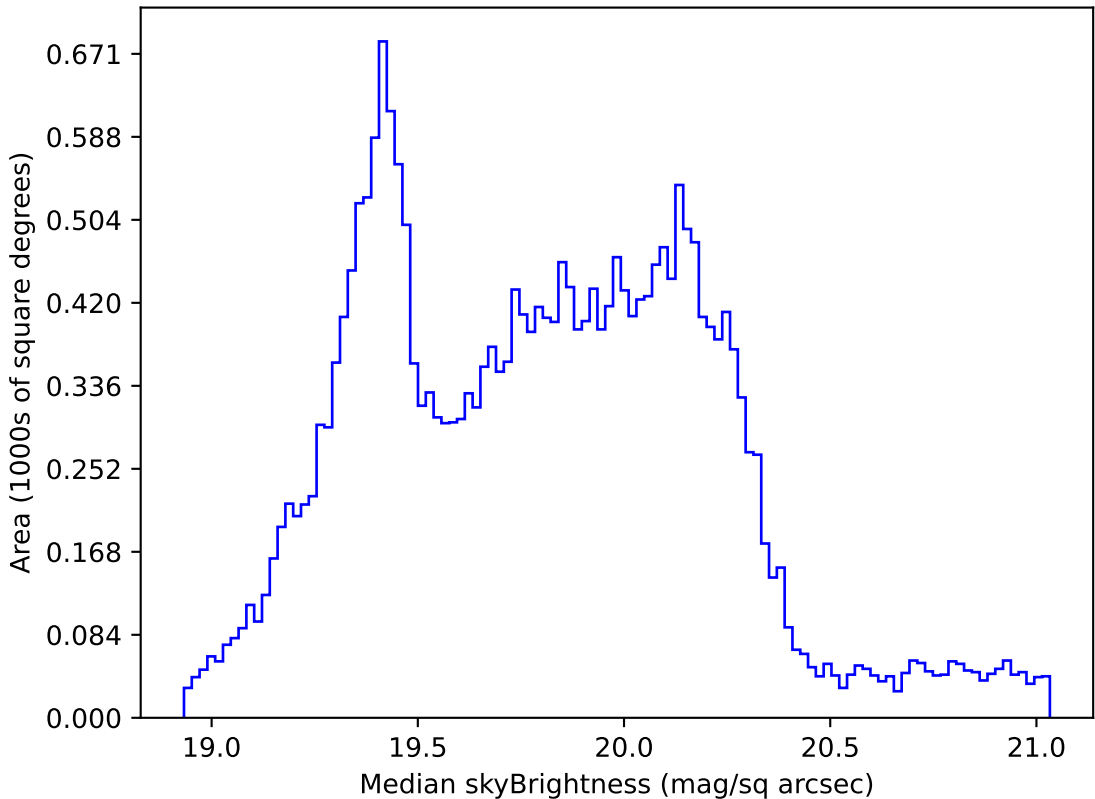
weather_cloudso0v3.5_10yrs Yr 1 all bands: Median skyBrightness
