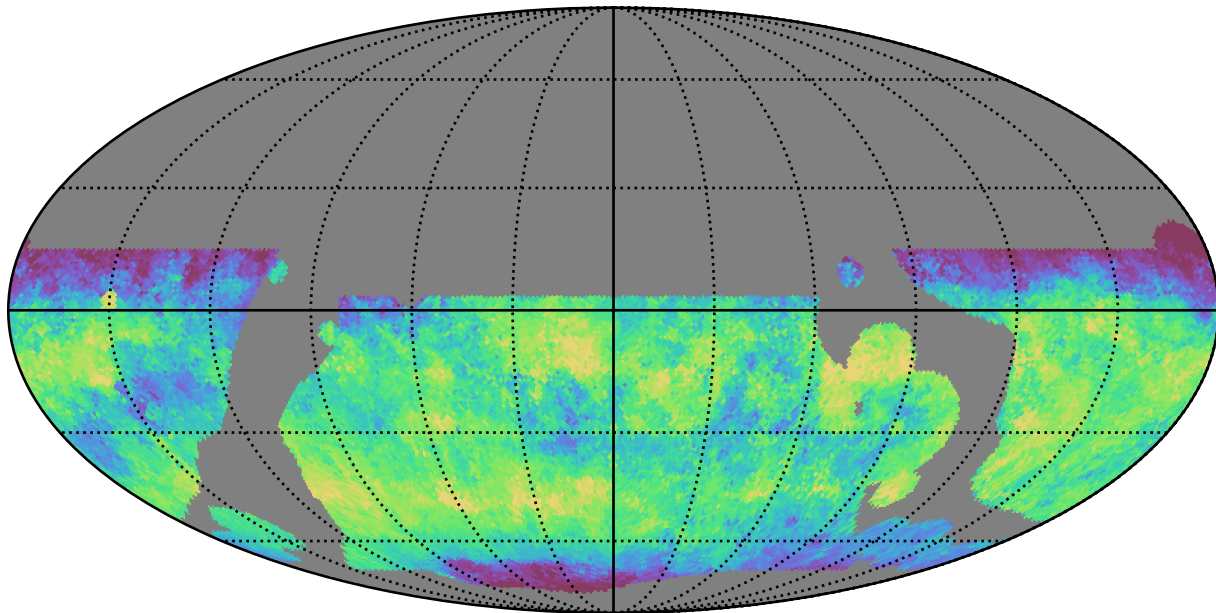
weather_cloudso0v3.5_10yrs WFD z band: Median skyBrightness
