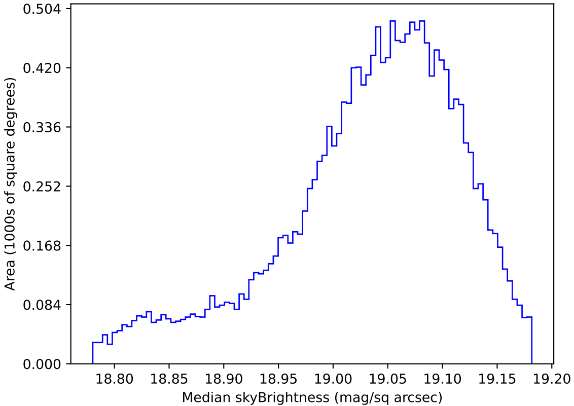
weather_cloudso0v3.5_10yrs WFD z band: Median skyBrightness
