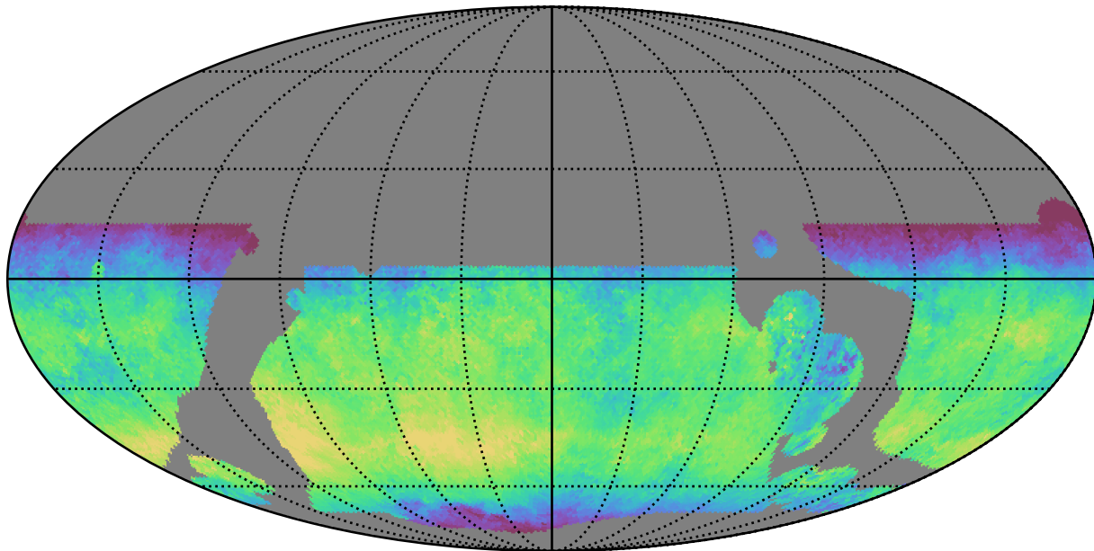
weather_cloudso0v3.5_10yrs WFD y band: Median skyBrightness
