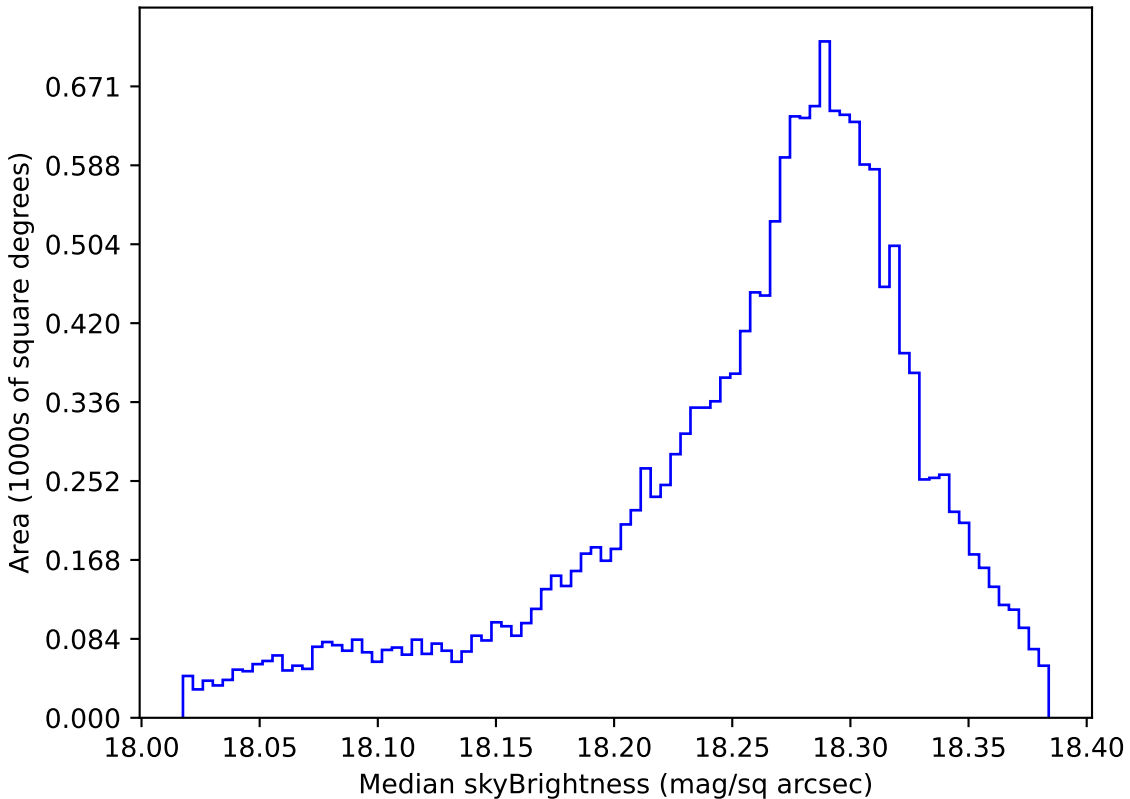
weather_cloudso0v3.5_10yrs WFD y band: Median skyBrightness
