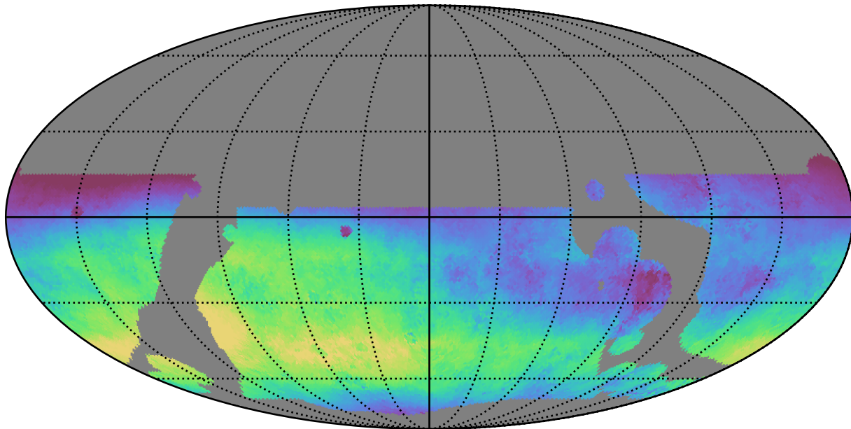
weather_cloudso0v3.5_10yrs WFD u band: Median skyBrightness
