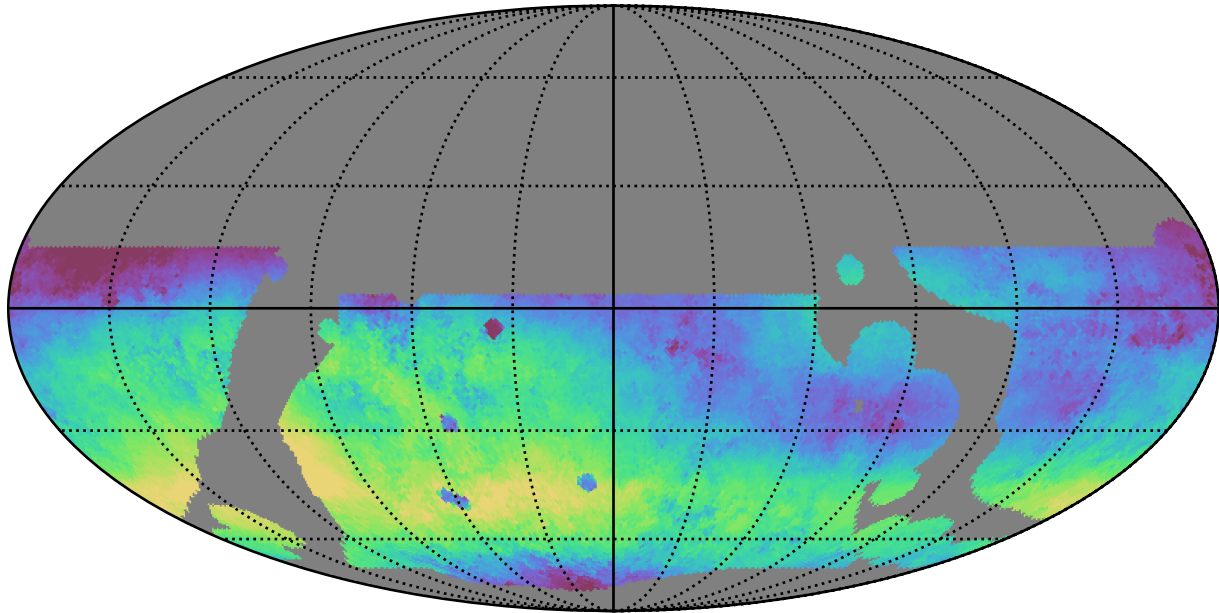
weather_cloudso0v3.5_10yrs WFD r band: Median skyBrightness
