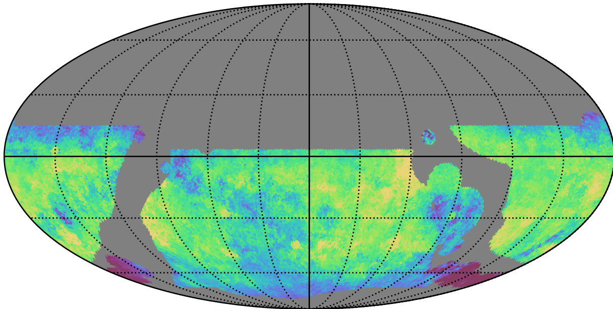
weather_cloudso0v3.5_10yrs WFD i band: Median skyBrightness
