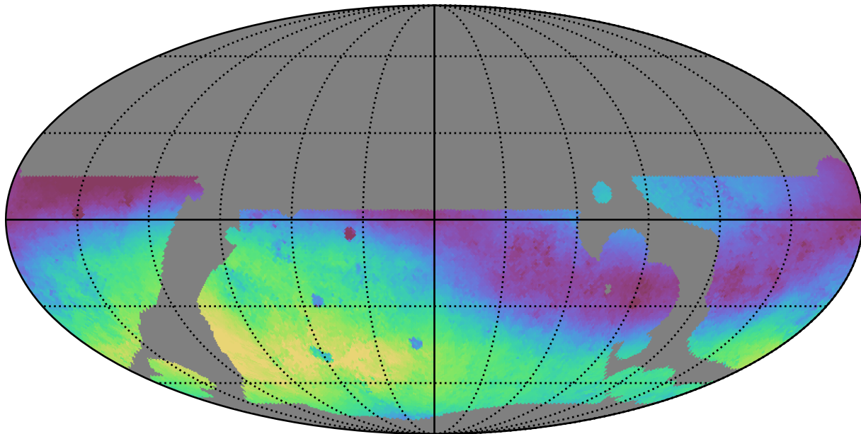
weather_cloudso0v3.5_10yrs WFD g band: Median skyBrightness
