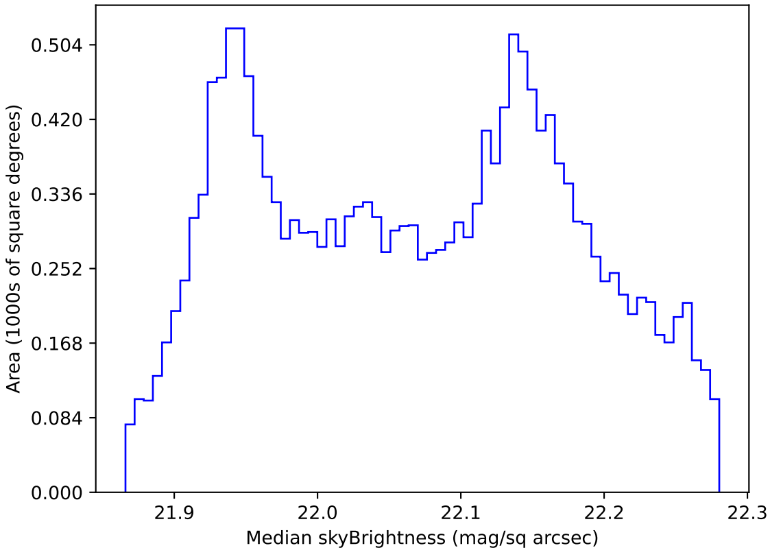
weather_cloudso0v3.5_10yrs WFD g band: Median skyBrightness
