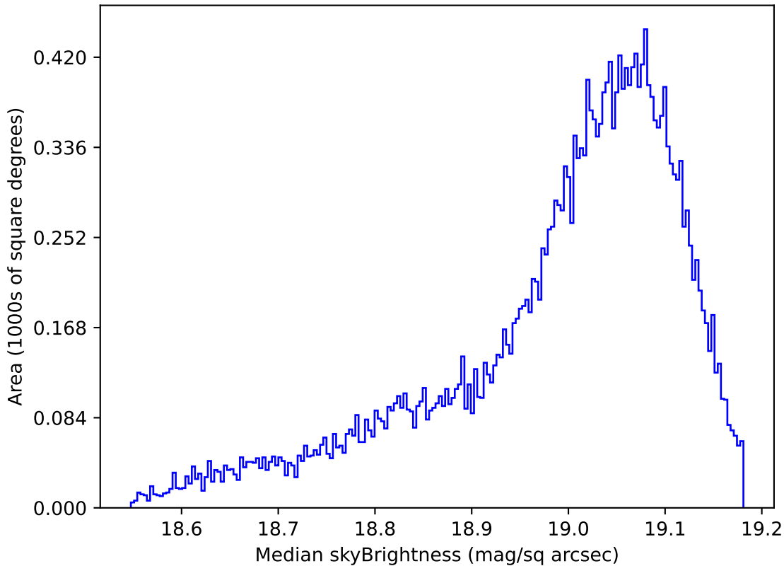
weather_cloudso0v3.5_10yrs All sky z band: Median skyBrightness
