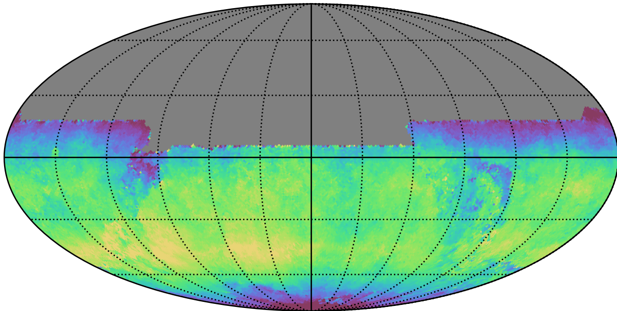
weather_cloudso0v3.5_10yrs All sky y band: Median skyBrightness
