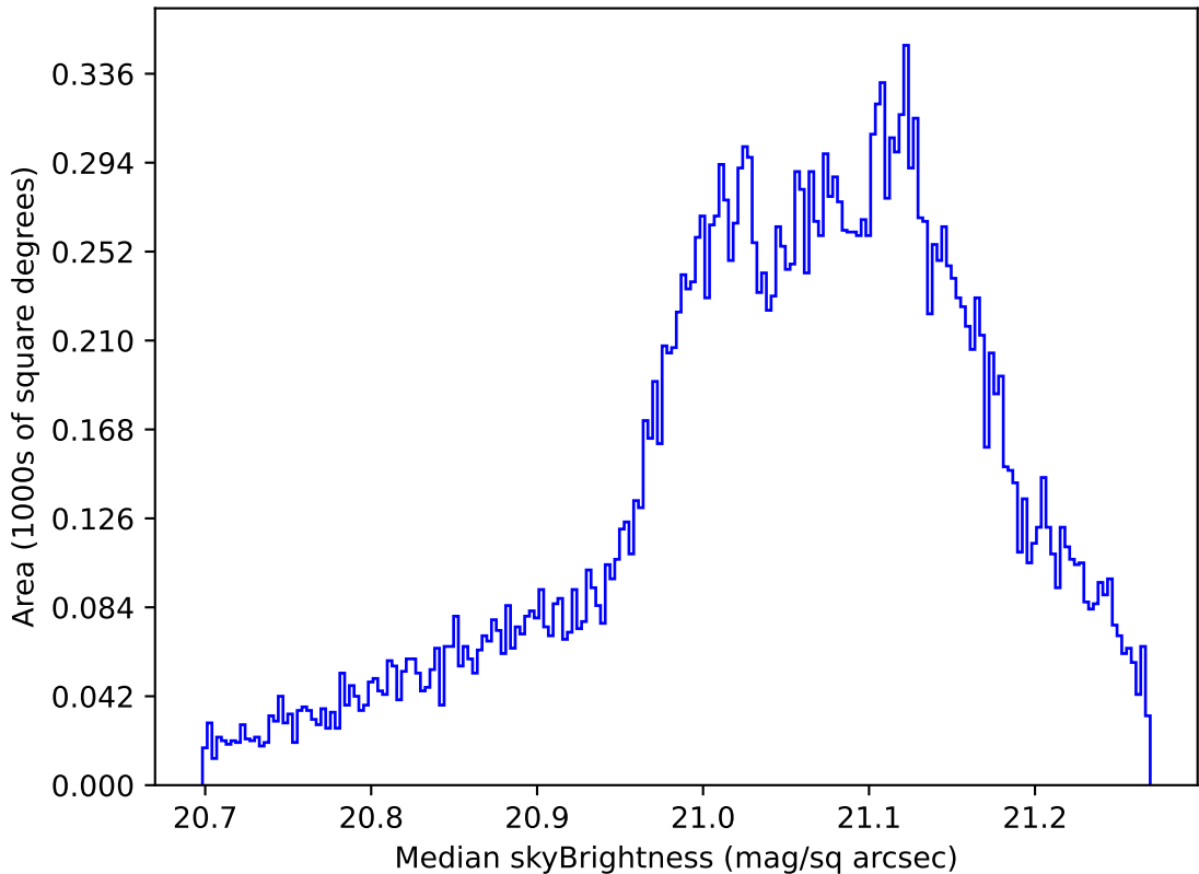
weather_cloudso0v3.5_10yrs All sky r band: Median skyBrightness
