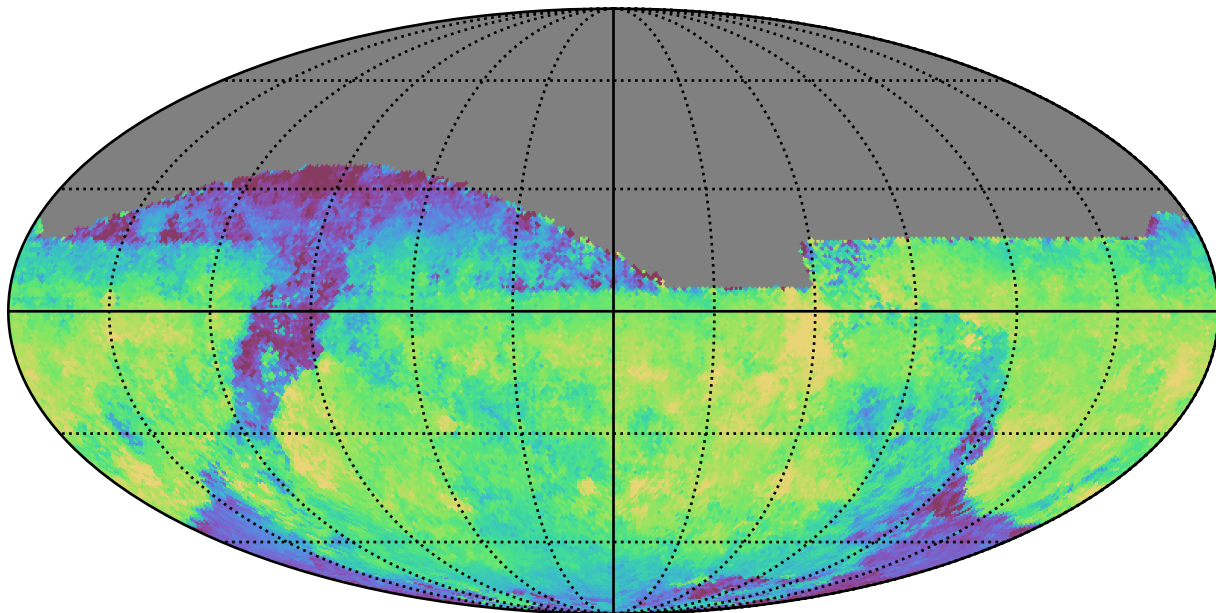
weather_cloudso0v3.5_10yrs All sky i band: Median skyBrightness
