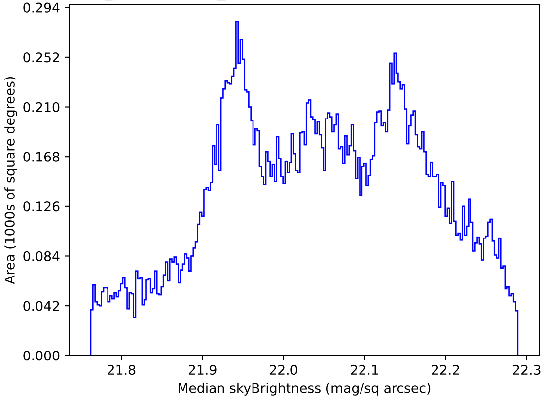
weather_cloudso0v3.5_10yrs All sky g band: Median skyBrightness
