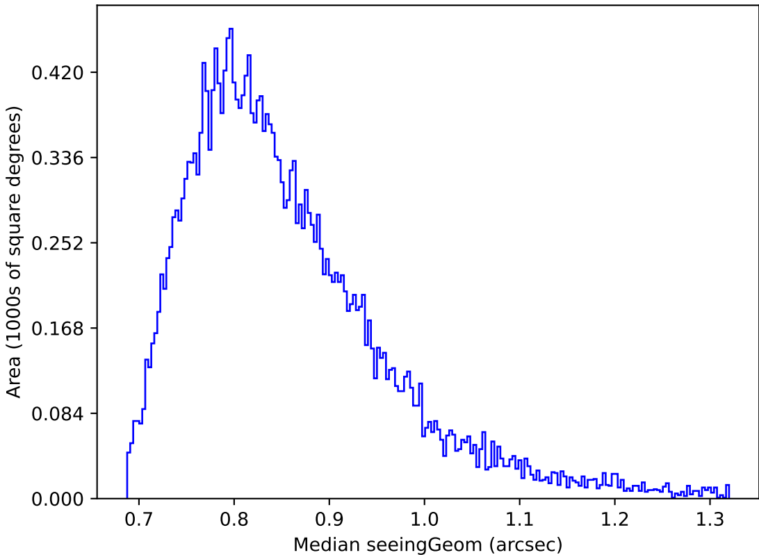
weather_cloudso0v3.5_10yrs Yr 1 z band: Median seeingGeom
