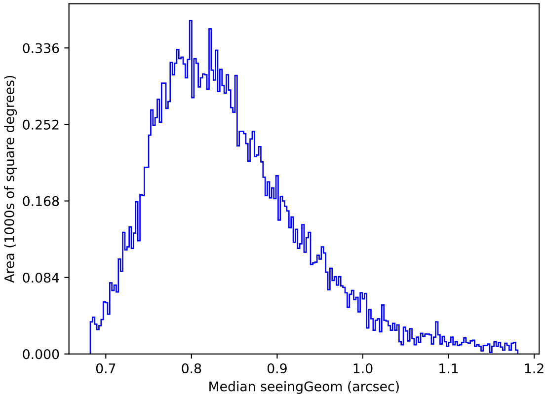
weather_cloudso0v3.5_10yrs Yr 1 y band: Median seeingGeom
