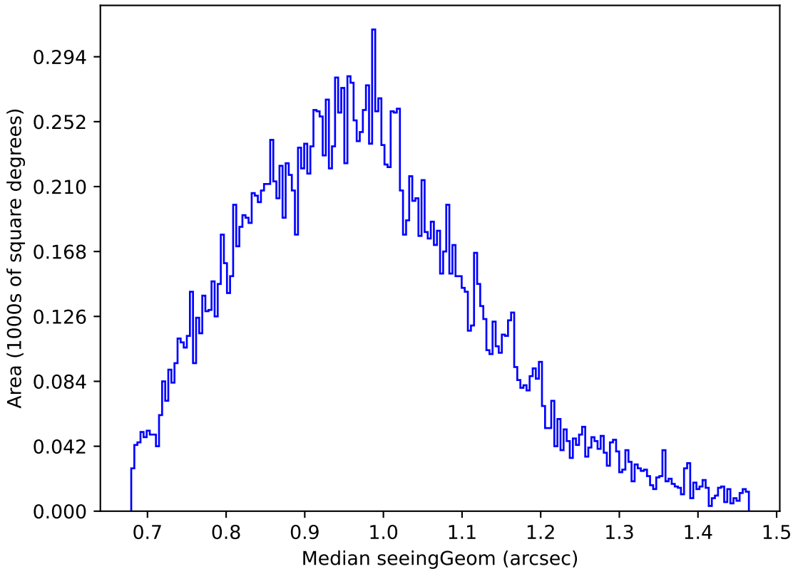
weather_cloudso0v3.5_10yrs Yr 1 u band: Median seeingGeom
