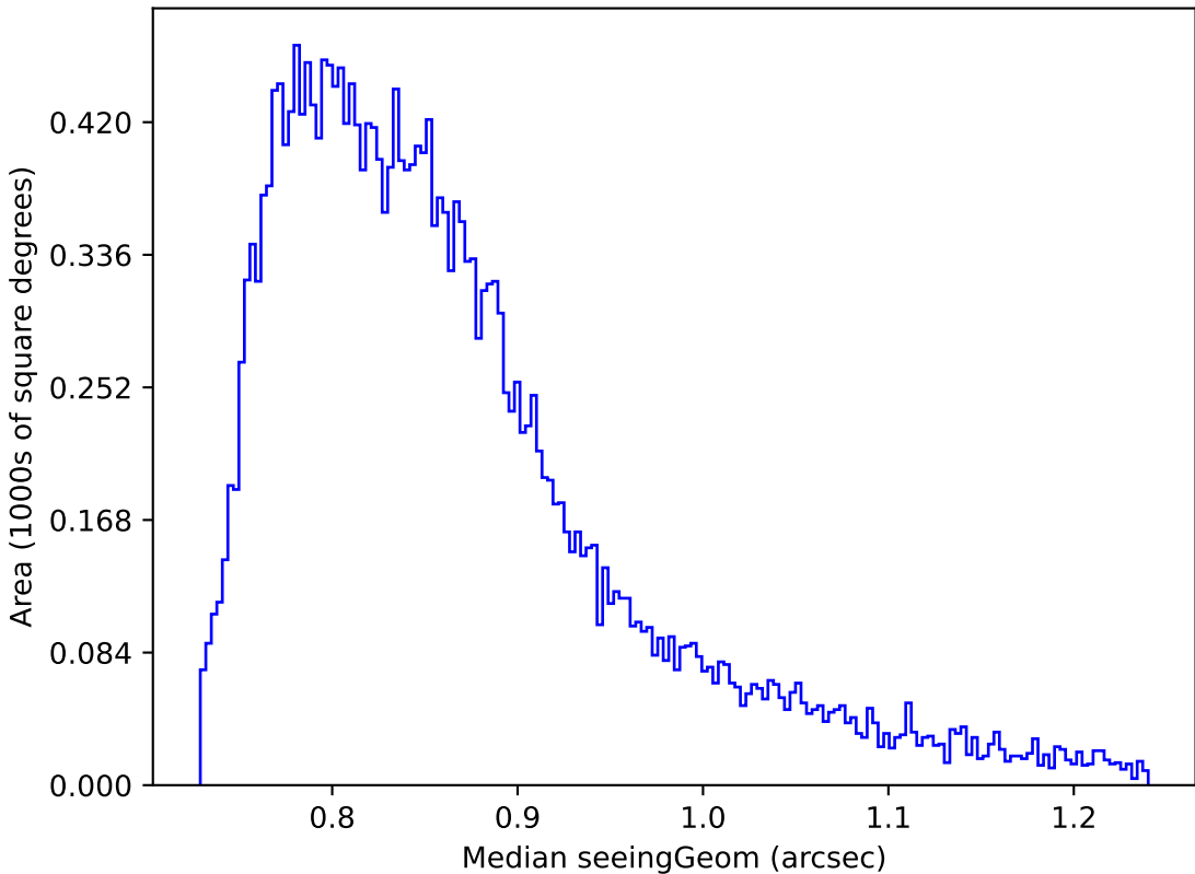
weather_cloudso0v3.5_10yrs Yr 1 all bands: Median seeingGeom
