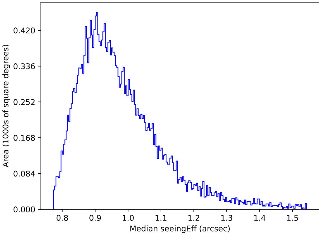
weather_cloudso0v3.5_10yrs Yr 1 z band: Median seeingEff
