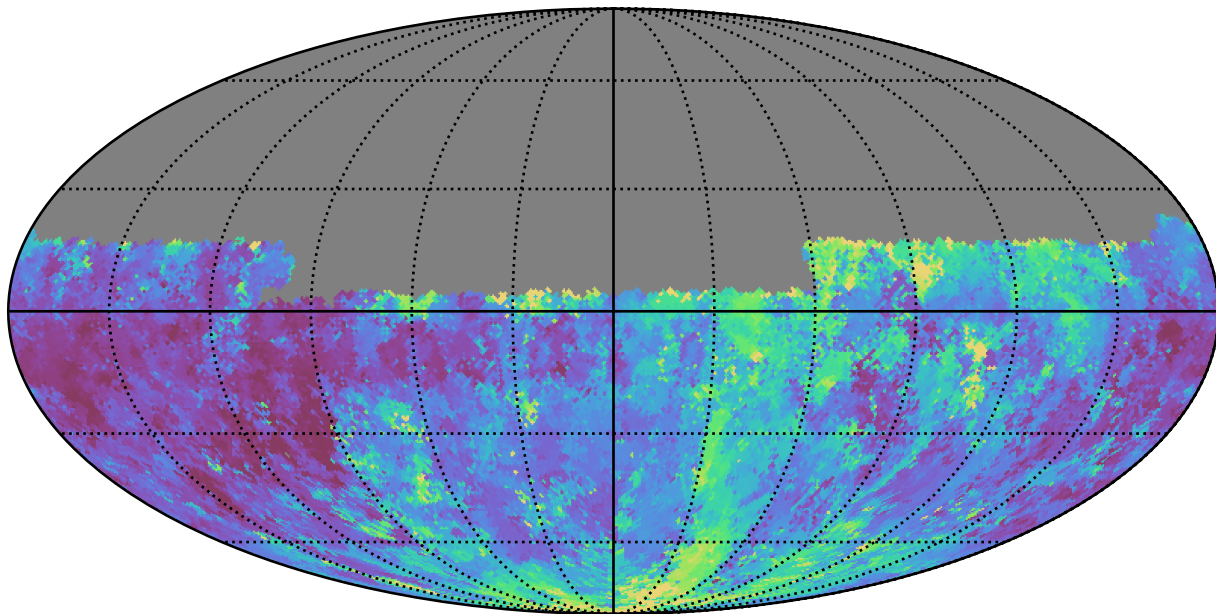
weather_cloudso0v3.5_10yrs Yr 1 u band: Median seeingEff
