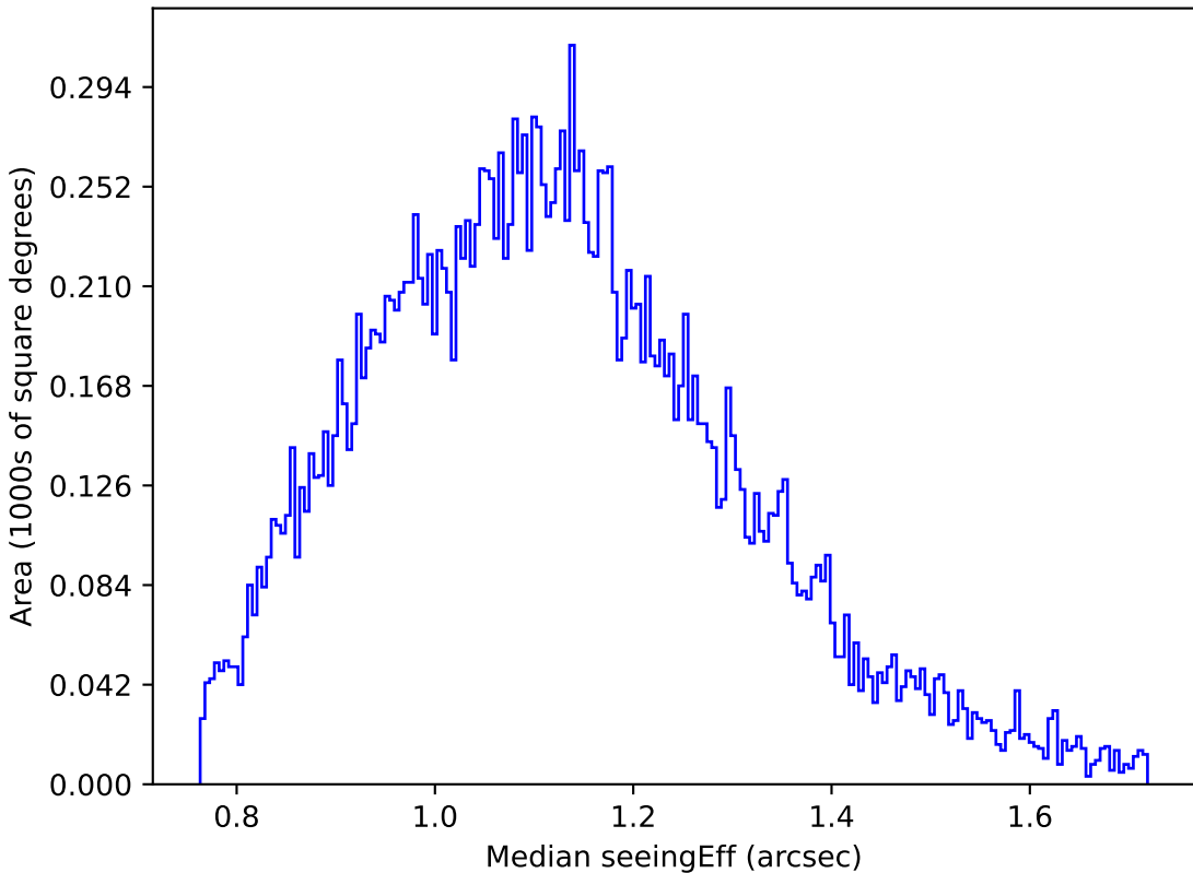
weather_cloudso0v3.5_10yrs Yr 1 u band: Median seeingEff
