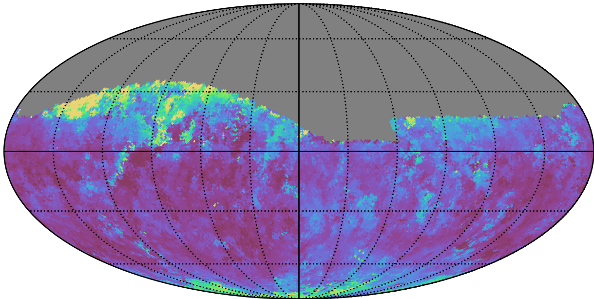
weather_cloudso0v3.5_10yrs Yr 1 i band: Median seeingEff
