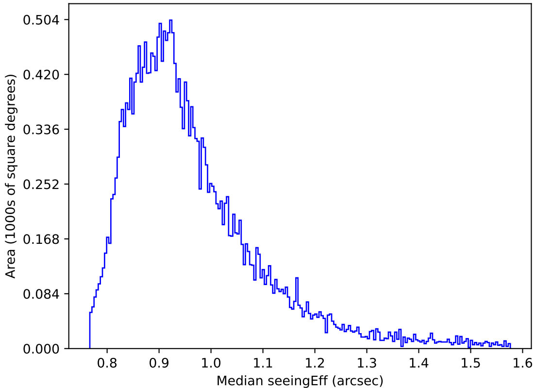
weather_cloudso0v3.5_10yrs Yr 1 i band: Median seeingEff
