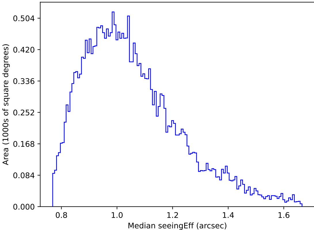
weather_cloudso0v3.5_10yrs Yr 1 g band: Median seeingEff
