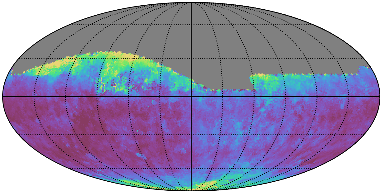
weather_cloudso0v3.5_10yrs Yr 1 all bands: Median seeingEff
