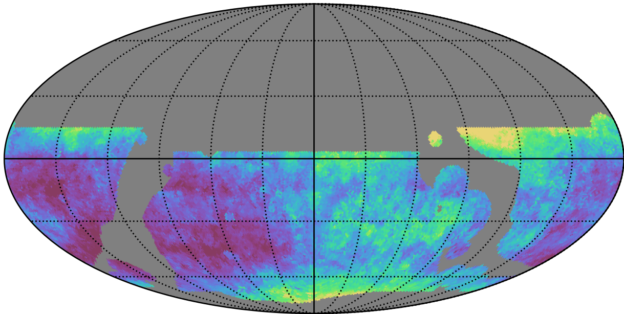
weather_cloudso0v3.5_10yrs WFD z band: Median seeingEff
