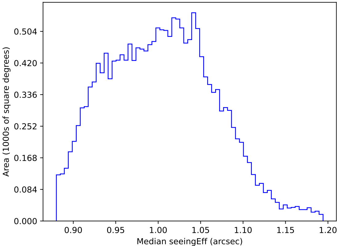
weather_cloudso0v3.5_10yrs WFD z band: Median seeingEff
