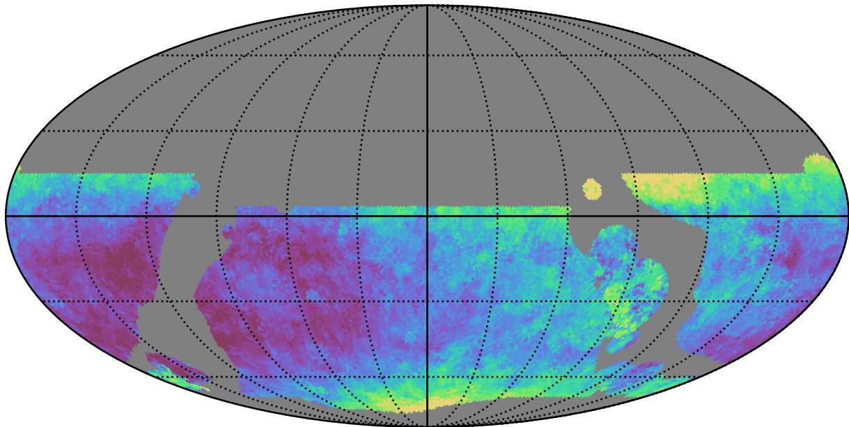
weather_cloudso0v3.5_10yrs WFD y band: Median seeingEff
