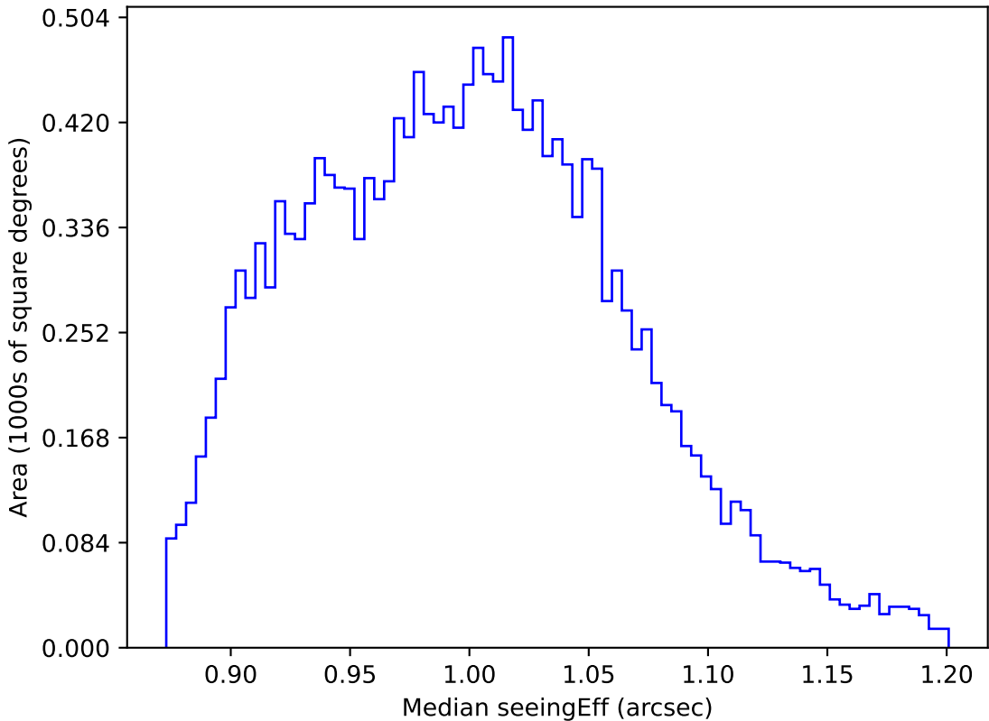
weather_cloudso0v3.5_10yrs WFD y band: Median seeingEff
