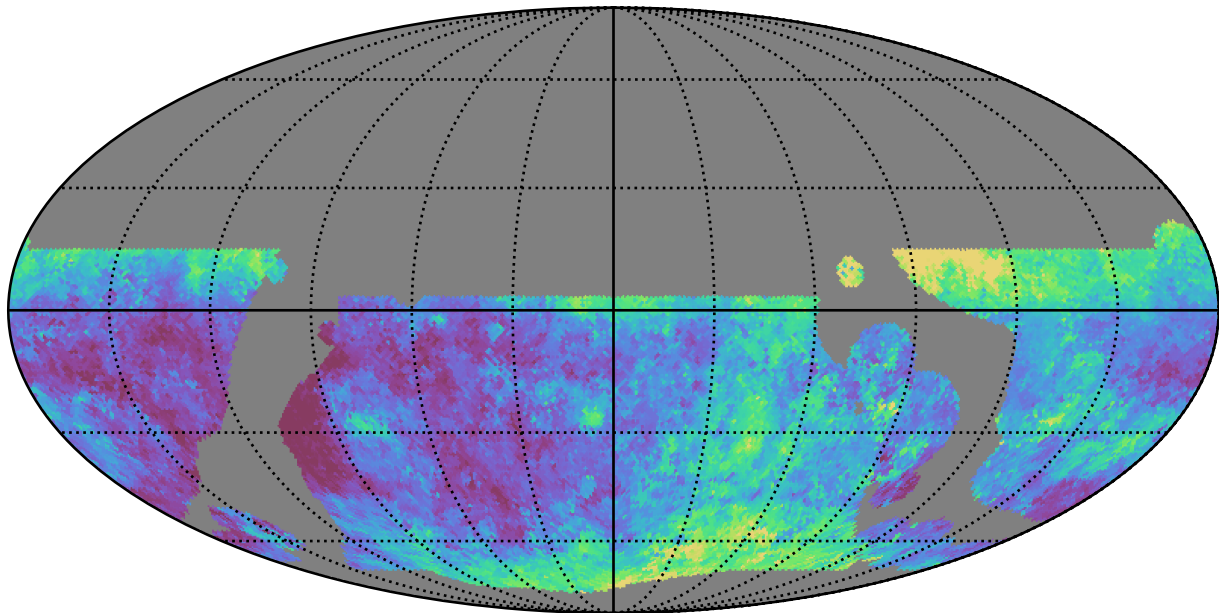
weather_cloudso0v3.5_10yrs WFD u band: Median seeingEff
