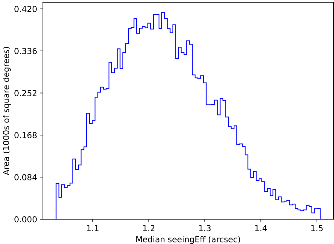
weather_cloudso0v3.5_10yrs WFD u band: Median seeingEff
