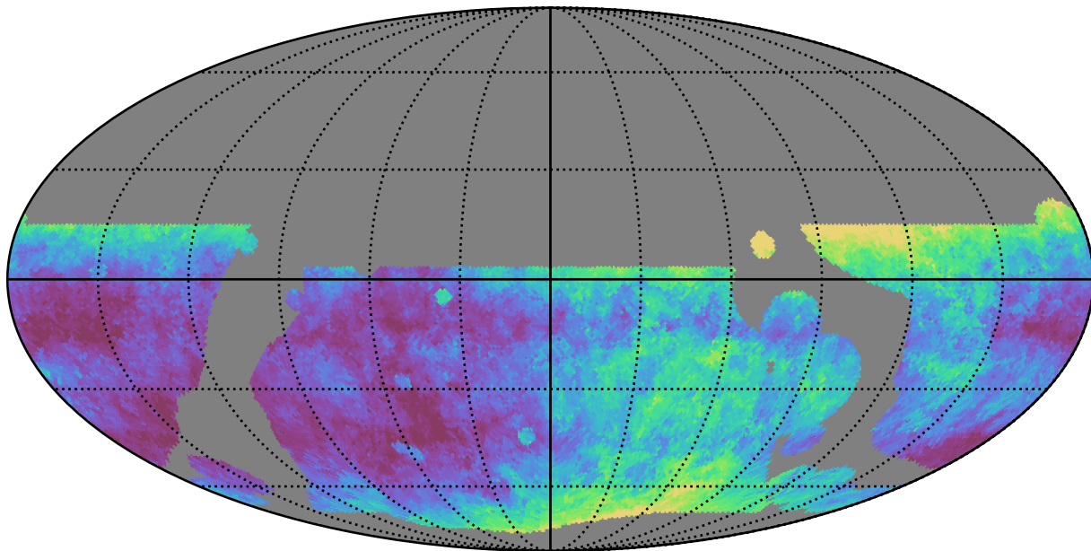
weather_cloudso0v3.5_10yrs WFD r band: Median seeingEff
