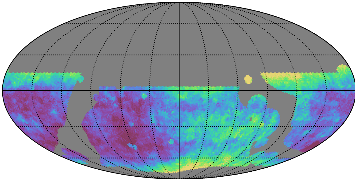
weather_cloudso0v3.5_10yrs WFD i band: Median seeingEff
