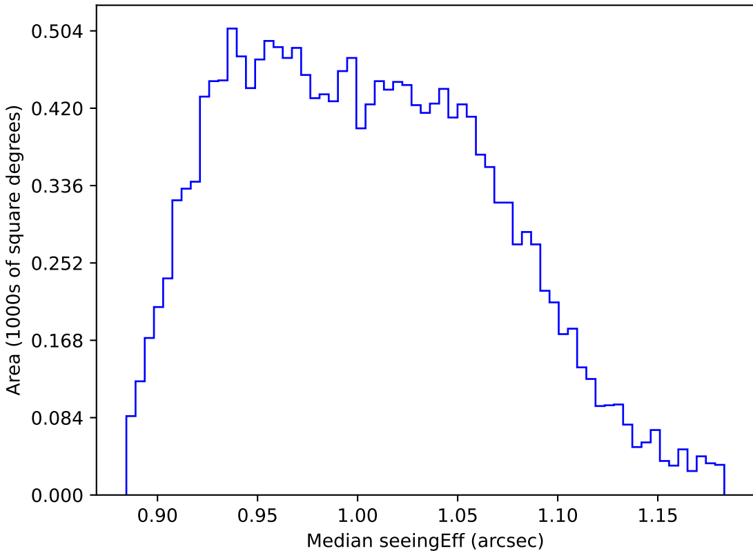
weather_cloudso0v3.5_10yrs WFD i band: Median seeingEff
